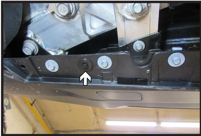
8b. Hybrid (4xe) Models: Remove one (1) push pin from the each side of the vehicle.
