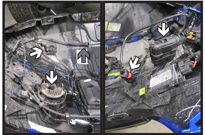
8c. Hybrid (4xe) Models: Remove fascia, disconnecting all electrical. There are two (2) electrical connections (white) on each side of the vehicle as well as a headlight cleaning hose (gray) on the passenger side. Set fascia aside to be reinstalled later.
