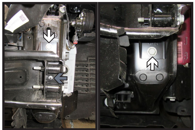
10. Using a 16MM socket, remove the two (2) bolts (white) from the bumper. Then using a 10MM socket, remove the one (1) nut (gray). Do this on both sides of the vehicle. Remove bumper and set aside. It will not be reinstalled later.
