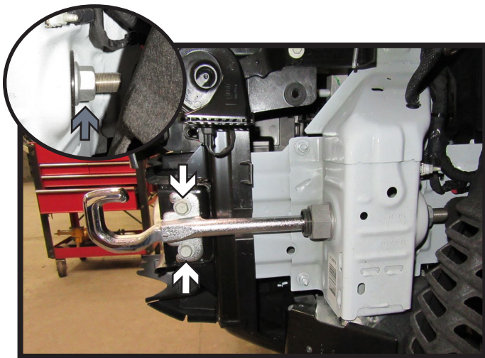
9. Using a 16MM socket, remove the two (2) bolts (white) from the tow hook. Then using a large crescent wrench, remove the nut (gray) from the back of the tow hook (inset). Remove tow hook and set aside to be reinstalled later. Do this on both sides of the vehicle.
